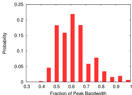
Figure 3: A visualization of a simulation with the hist_acc_band metric: the probability distribution for the bandwidth achieved by a bisection bandwidth measurement pattern for a random mapping—it can be observed that the mapping has a large impact on the resulting performance.
