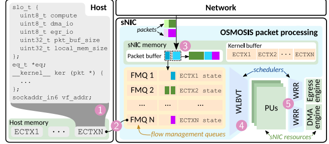
Figure 6: Abstract model of OSMOSIS-enabled sNIC. Packets are mapped by Matching Engine to FMQs and dispatched for execution by the scheduler.
